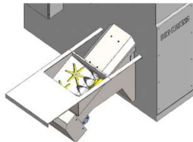
SLIDING HATCH
