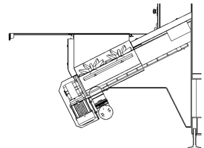
SECTION VIEW
